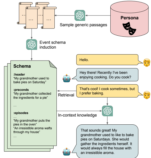
Figure 1: A diagram of our approach. (1) Given an unstructured persona dataset, we first sample “generic passages” from the facts in the persona, and then induce structured event schemas from the sampled stories. (2) We condition an LLM to generate dialogue responses that are fluent with previous conversation – yet that make use of the rich knowledge contained in the resulting schemas – by first using a retrieval model to select a relevant schema, and then providing the schema to the LLM as in-context knowledge.
