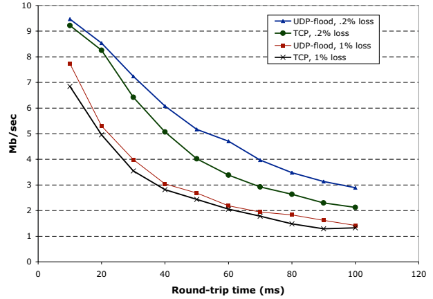
Figure 4: UDP Flood versus NewReno TCP: the STP policer restricts a UDP flow’s throughput to within 36% of TCP’s on a 10 Mbps link.
