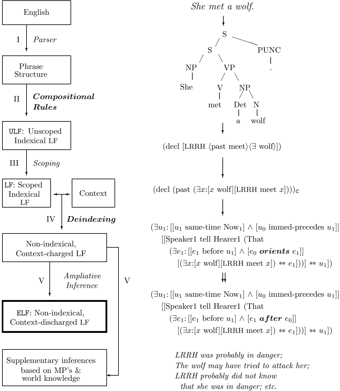
Fig. 2. The Conceptual Stages of NL Understanding
