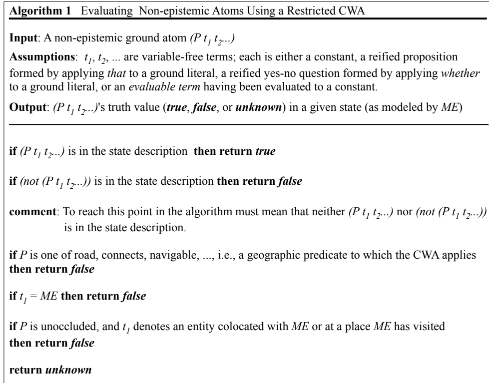
FIGURE 4. Evaluating Non-epistemic Atoms Using a Restricted CWA
