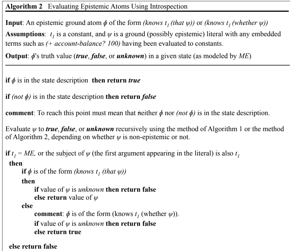
FIGURE 5. Evaluating Epistemic Atoms Using Introspection
