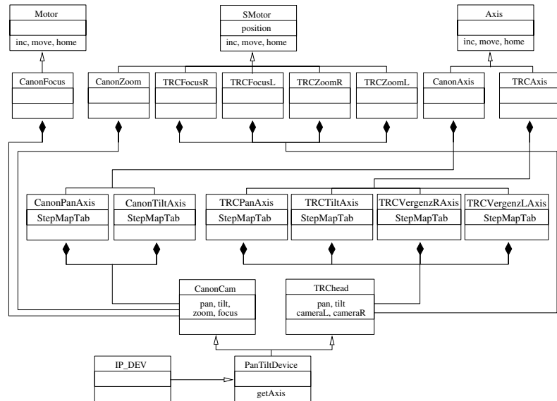
Figure 3. Class hierarchy for motors used in active vision systems.
